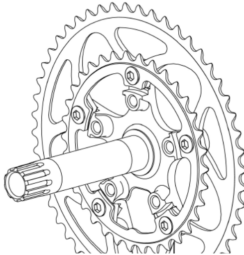
OX801D-PCD110mm "Compact Drive"
