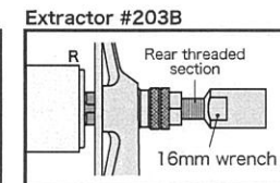
Extractor #203B
